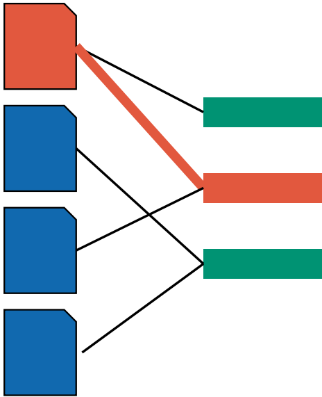
Term-document bipartite graph
